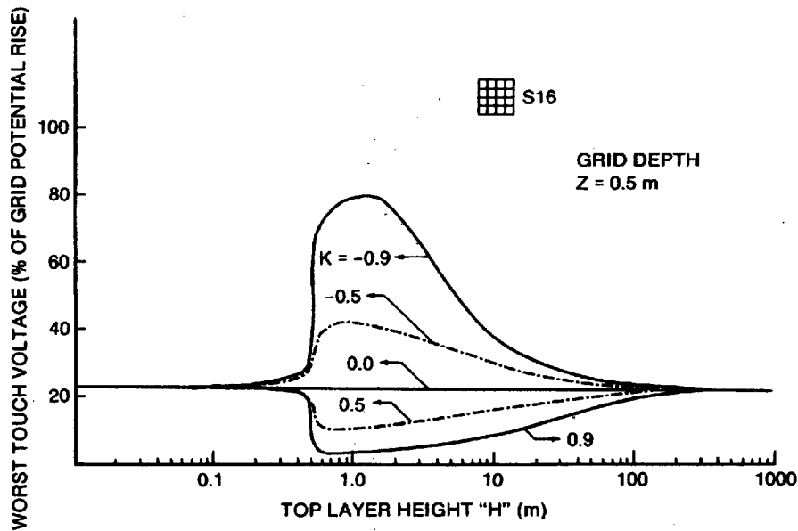
Figure F.7—Sixteen mesh grid touch voltages
