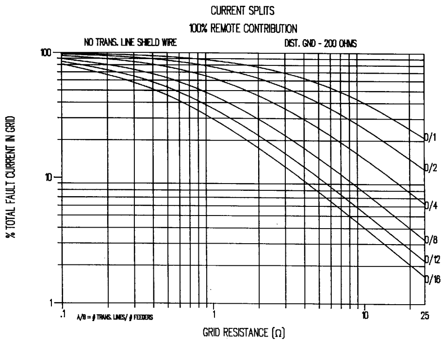
Figure C.16—Curves to approximate split factor S_f
