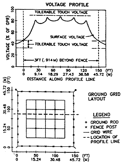
Figure 45—Case 5, plot 1
