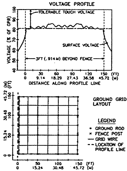
Figure 39—Case 2, plot 1
