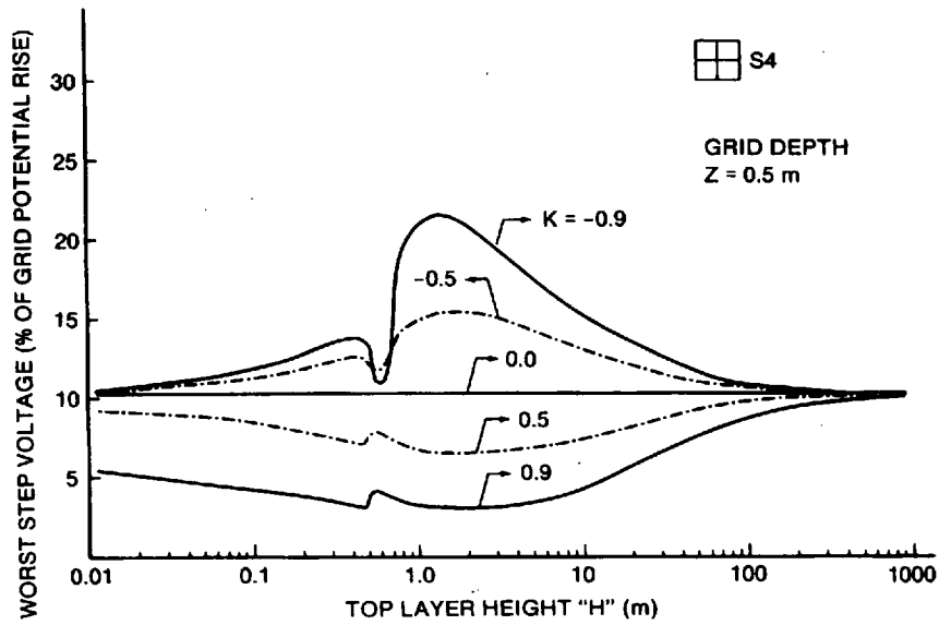
Figure F.8—Four mesh grid step voltages
