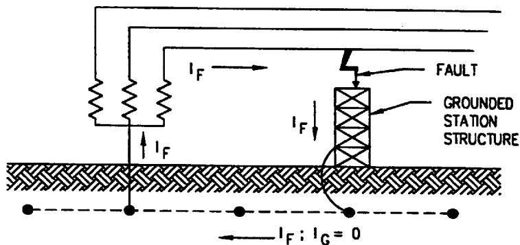
Figure 28—Fault within local substation; local neutral grounded
