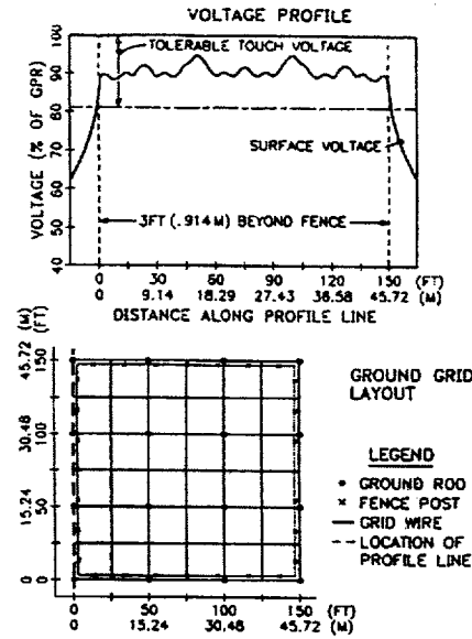
Figure 37—Case 1, plot 1
