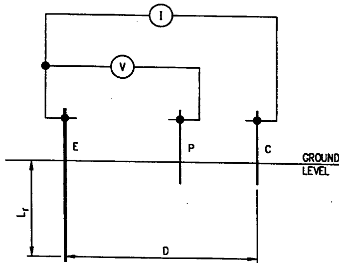
Figure 20—Circuit diagram for three-pin or driven-ground rod method
