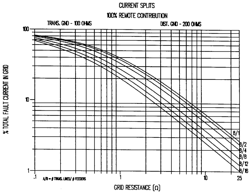
Figure C.8—Curves to approximate split factor S_f
