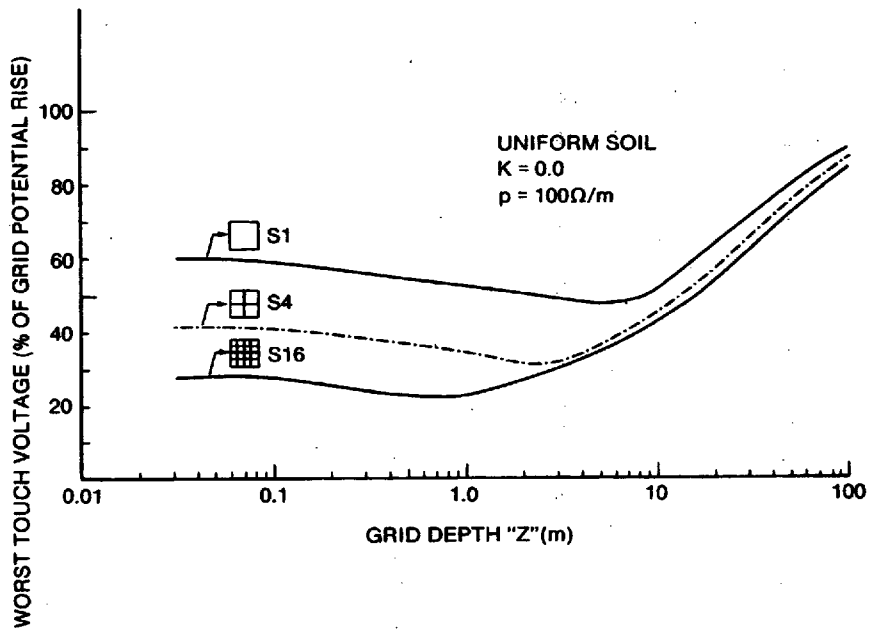
Figure F.10—Touch voltage versus grid depth
