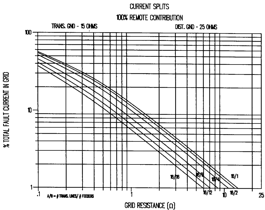
Figure C.11—Curves to approximate split factor S_f
