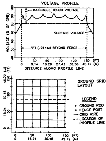
Figure 39—Case 2, plot 1
