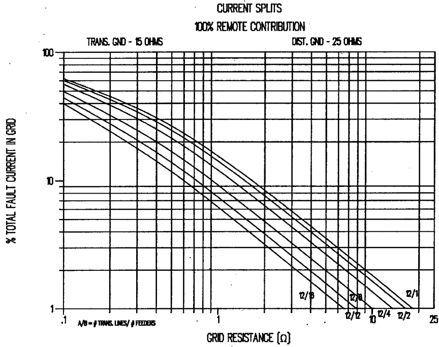
Figure C.9—Curves to approximate split factor S_f
