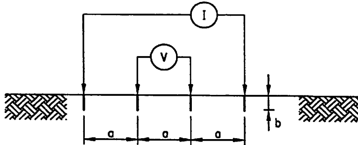
Figure 19—Wenner four-pin method
