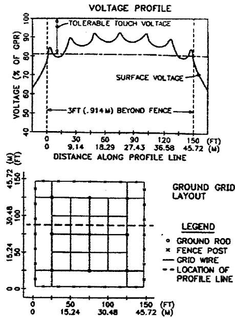
Figure 43—Case 4, plot 1
