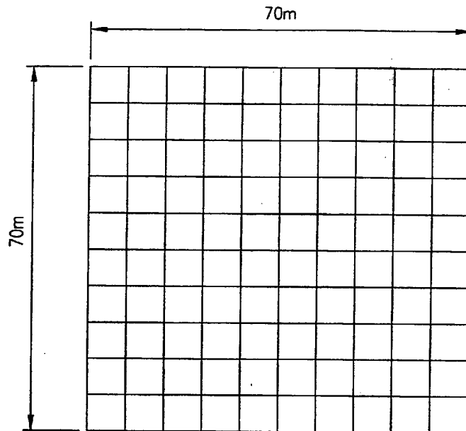
Figure B.1—Square grid without ground rods
