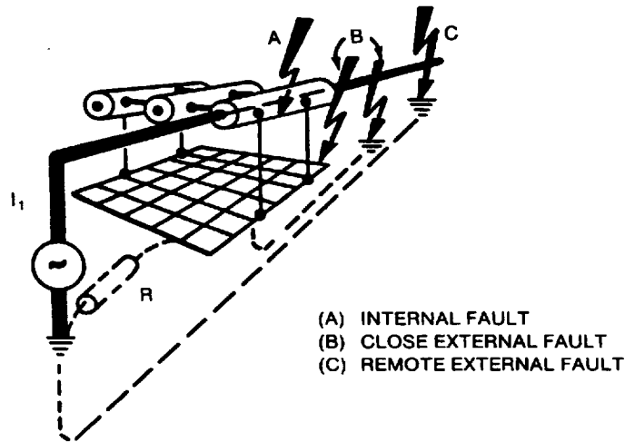
Figure 16—Typical faults in GIS
