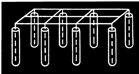
Figure 27—Grid with encased vertical electrodes
