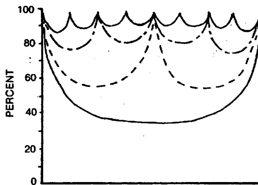
Figure G.6—Potential distribution for a ground mat with various mesh densities; ground mat potential = 100%
