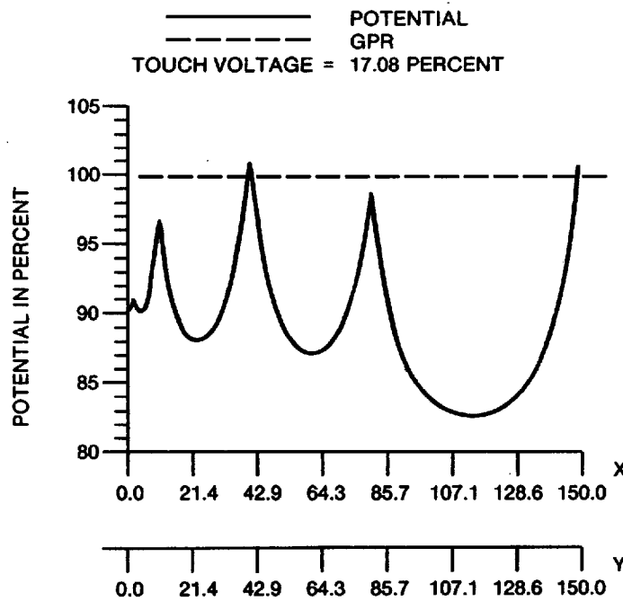
Figure B.8—Diagonal voltage profile for an unequally spaced grid of Figure B.7
