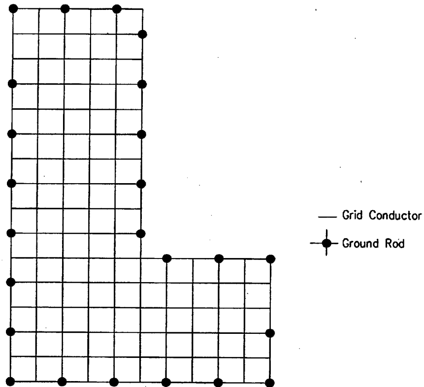
Figure B.4—L-shaped grid with twenty-four 7.5 m ground rods
