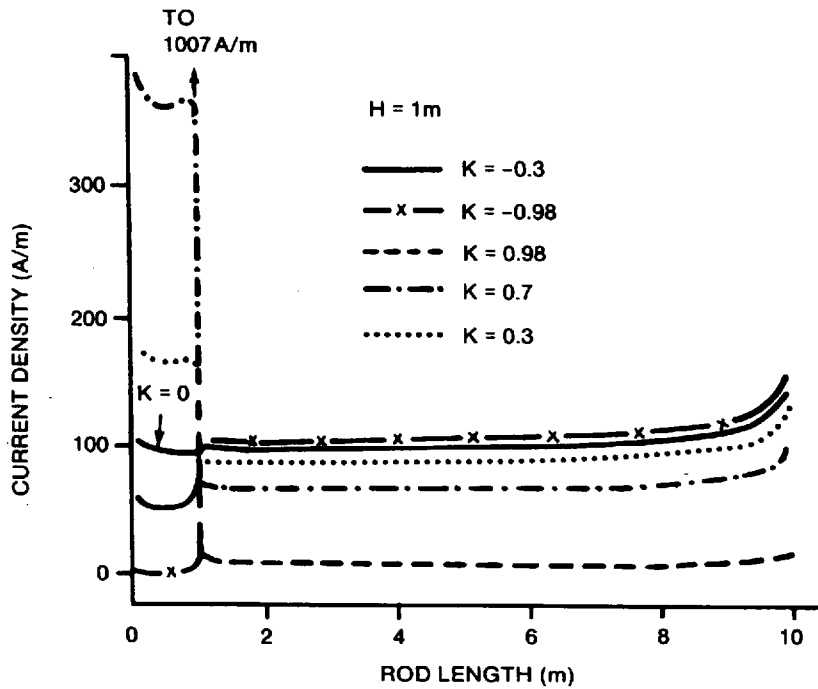
Figure F.12—Single rod current density
