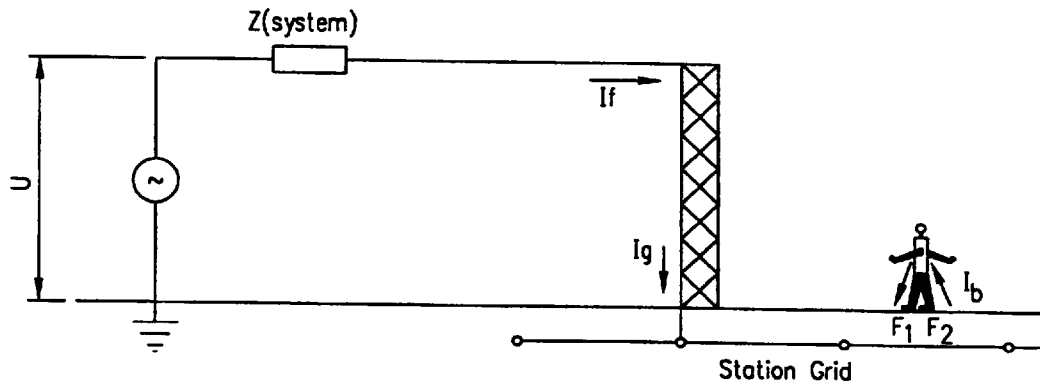
Figure 9—Exposure to step voltage
