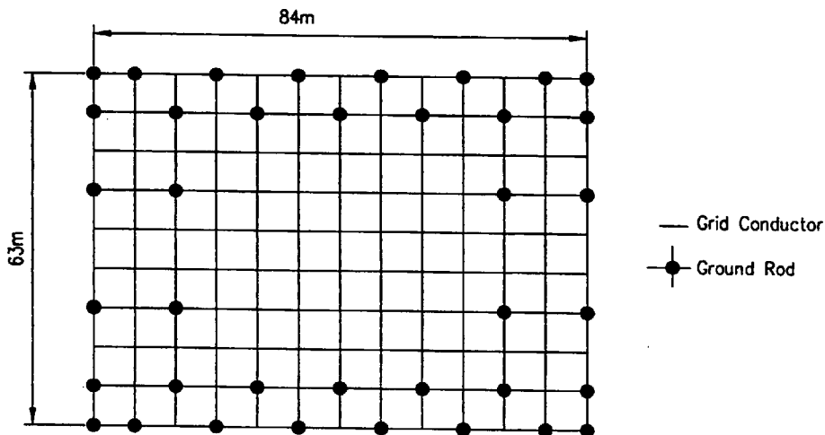
Figure B.3—Rectangular grid with thirty-eight 10 m ground rods
