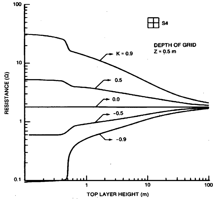
Figure F.3—Four mesh grid resistance
