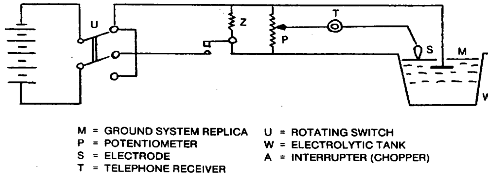
Figure G.1—Circuit for obtaining potential distribution
