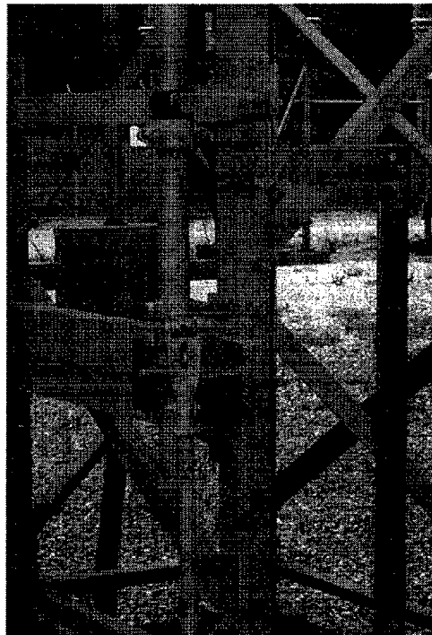
Figure 36—Typical braidless grounding device
