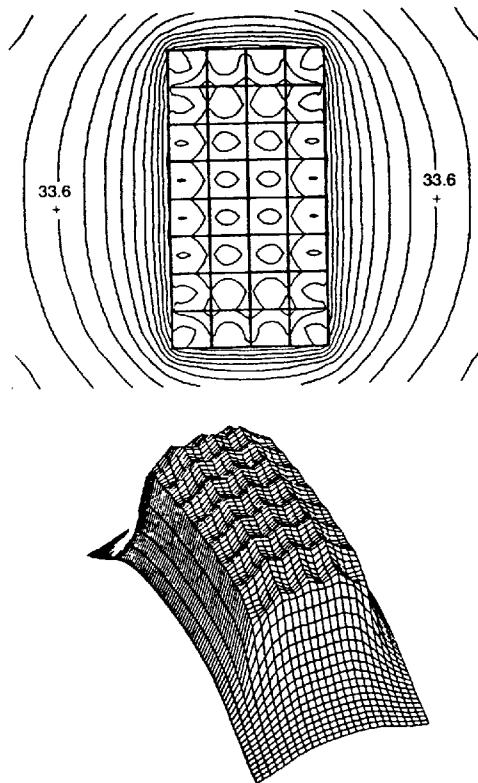
Figure 3—Equipotential contours if a typical grounding grid with and without ground rods
