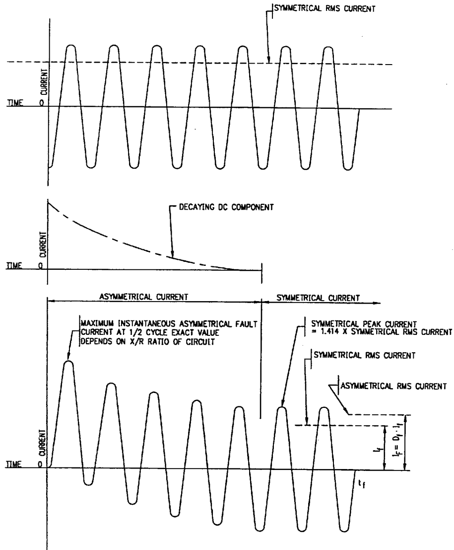
Figure 1—Relationship between actual values of fault current and values of I_F , I_f , and D_f for fault duration t_f
