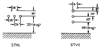
Figure C.24—System and configuration data for example 2 of C.3
