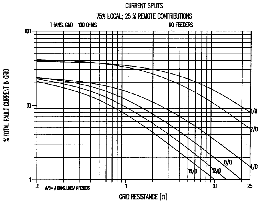
Figure C.22—Curves to approximate split factor S_f
