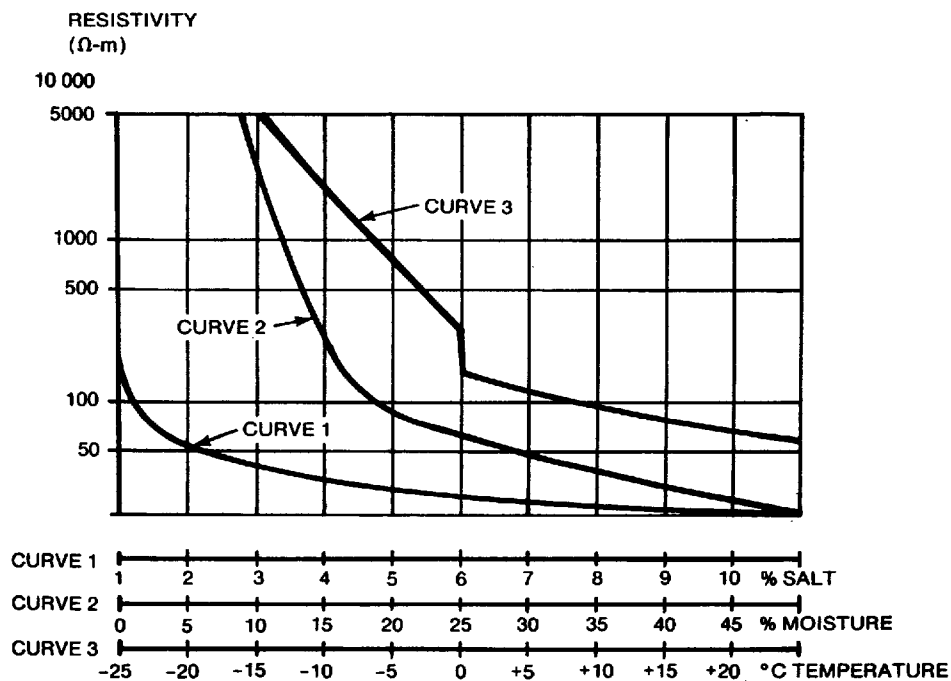
Figure 18—Effects of moisture, temperature, and salt upon soil resistivity
