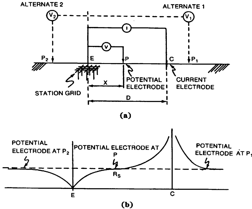
Figure 48—(a) Fall of potential method and (b) Earth surface potentials for various spacings “X”
