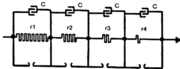
Figure 17—Soil model
