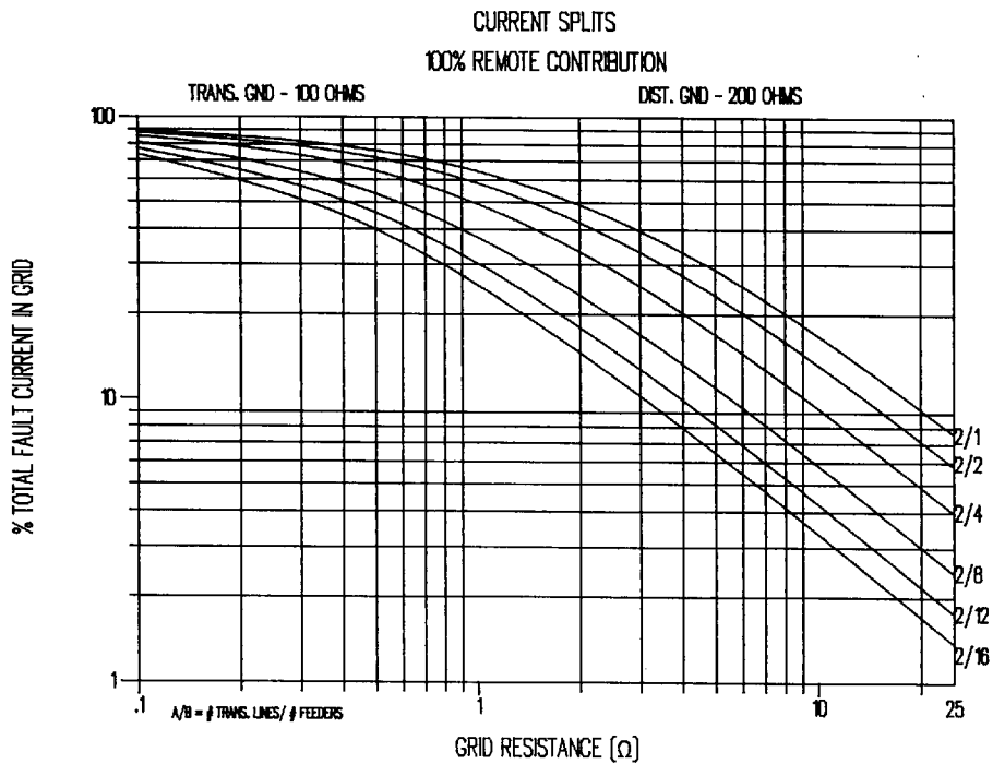
Figure C.4—Curves to approximate split factor S_f
