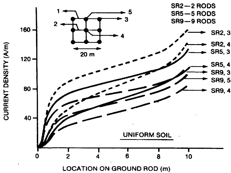
Figure F.16—Rod current density—rods and grids in uniform soil
