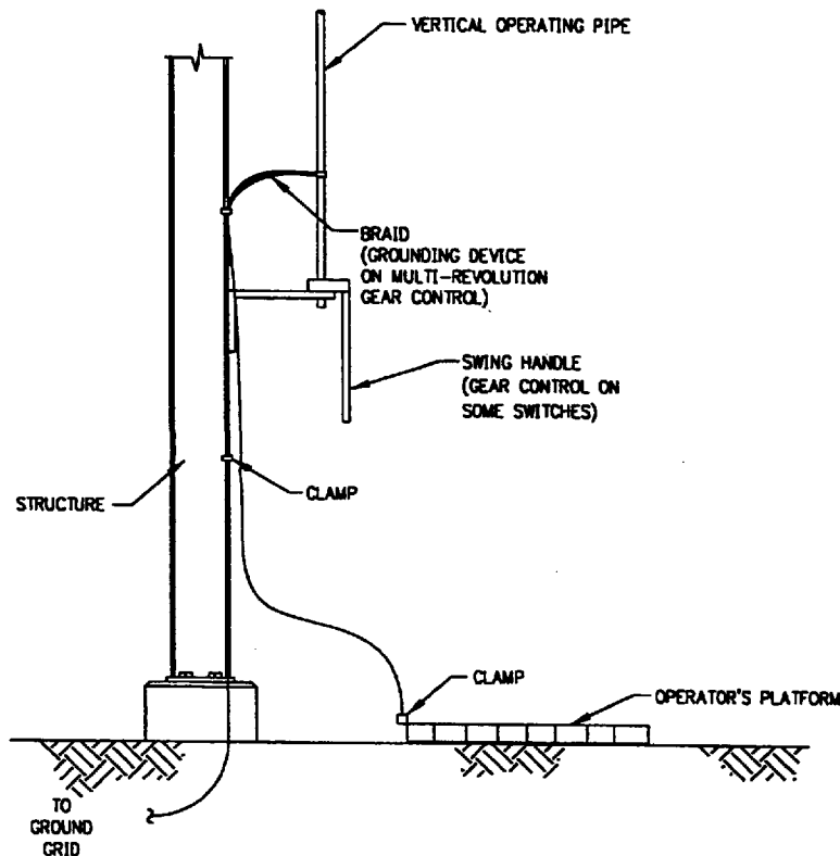
Figure 34—Typical switch shaft grounding
