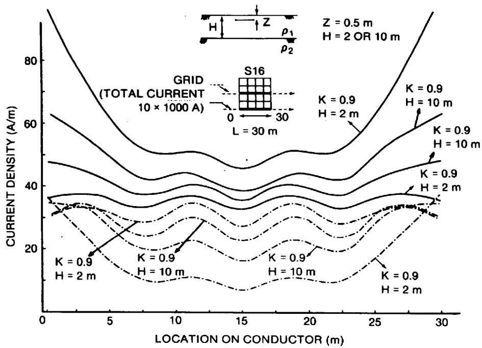
Figure F.2—Sixteen mesh grid current density
