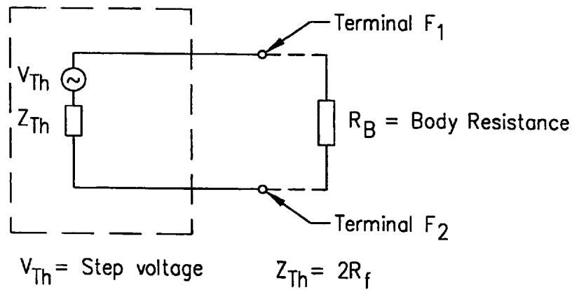
Figure 10—Step voltage circuit
