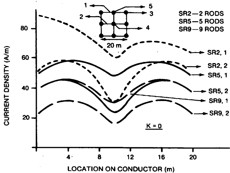
Figure F.15—Grid current density—rods and grid in uniform soil
