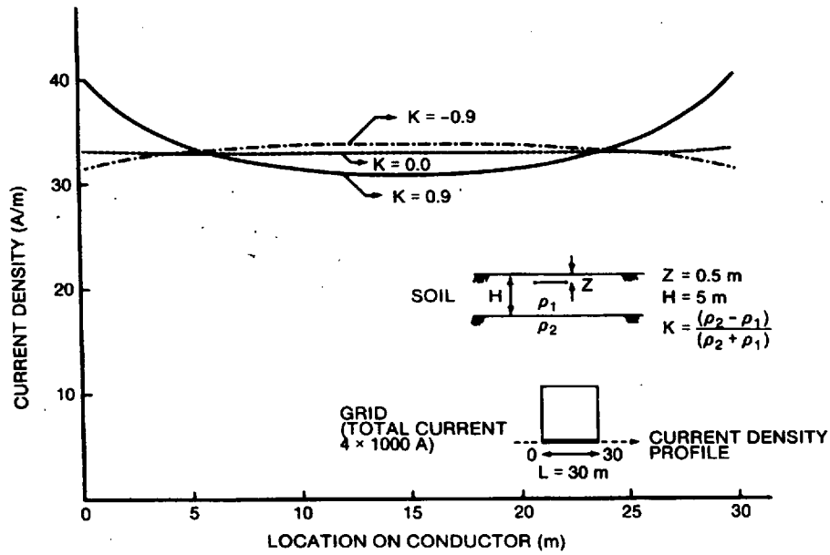
Figure F.1—One mesh grid current density
