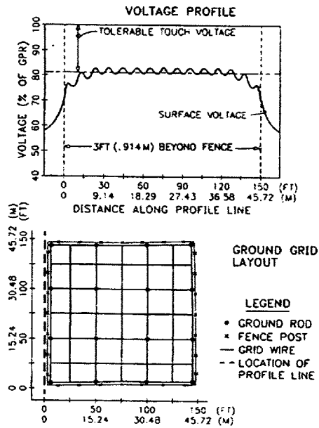
Figure 41—Case 3, plot 1
