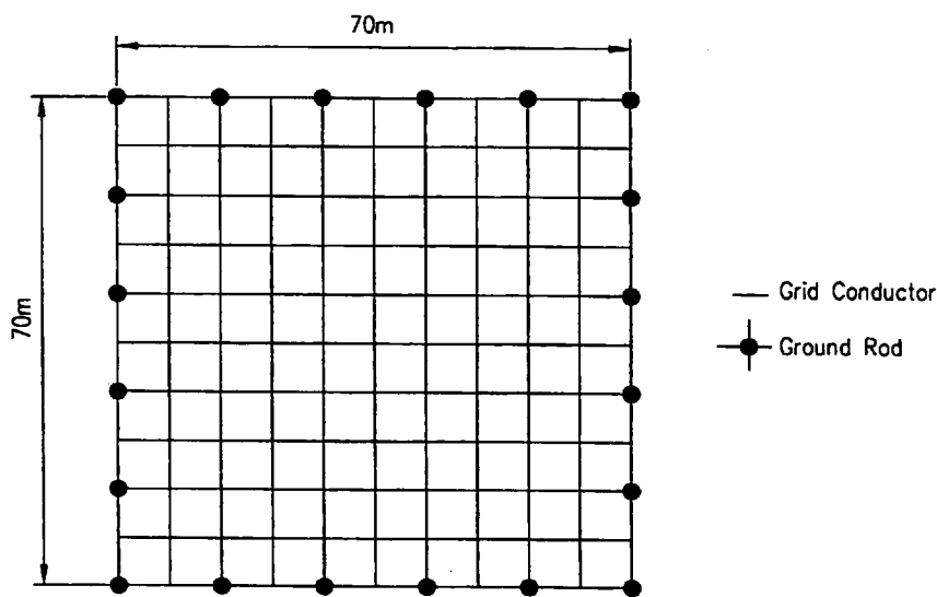
Figure B.2—Square grid with 20 7.5 m rods
