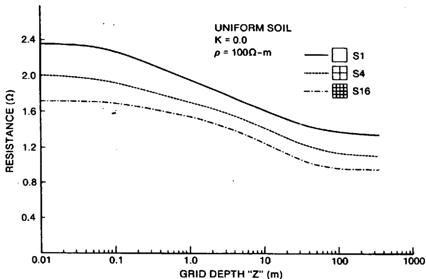
Figure F.5—Grid resistance versus grid depth
