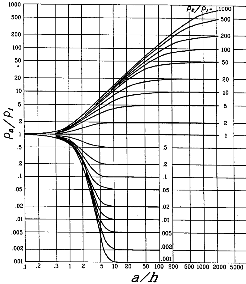
Figure 21—Sunde's graphical method
