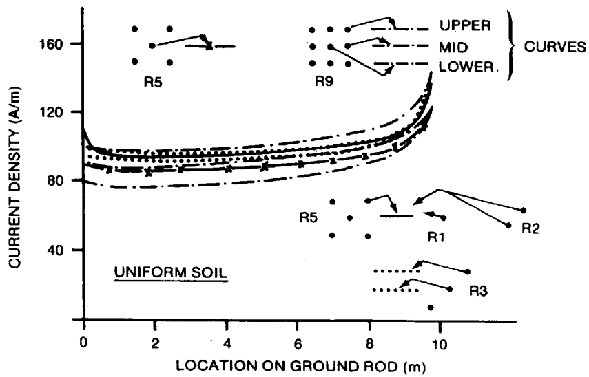
Figure F.13—Multiple driven rod current density in uniform soil
