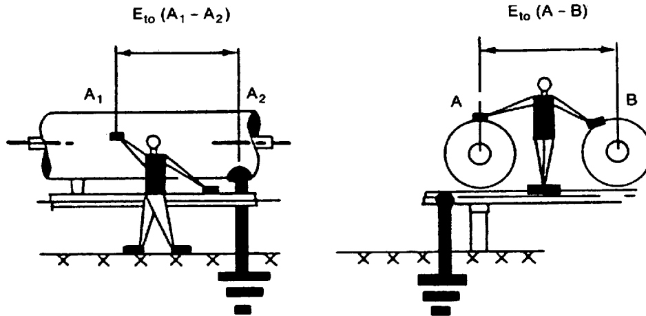
Figure 14—Typical metal-to-metal touch situation in GIS
