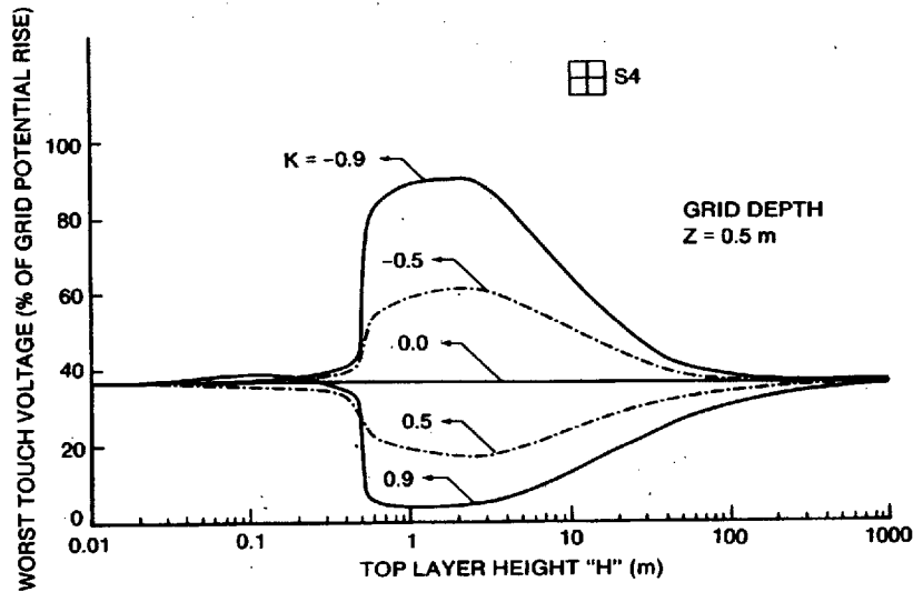
Figure F.6—Four mesh grid touch voltages
