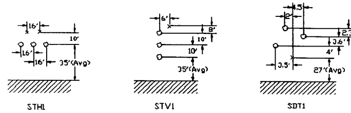
Figure C.23—System and configuration data for example 1 of C.3
