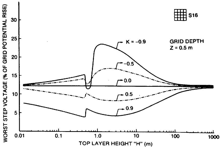
Figure F.9—Sixteen mesh grid step voltages
