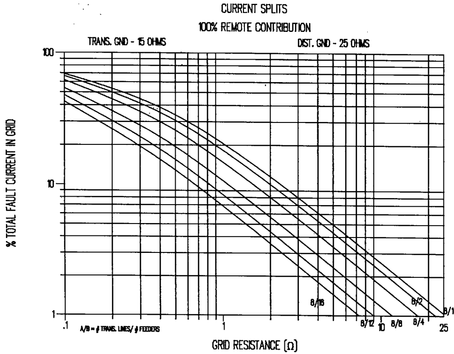
Figure C.7—Curves to approximate split factor S_f
