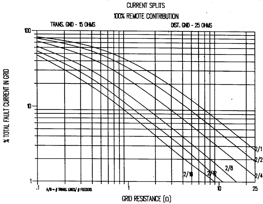
Figure C.3—Curves to approximate split factor S_f
