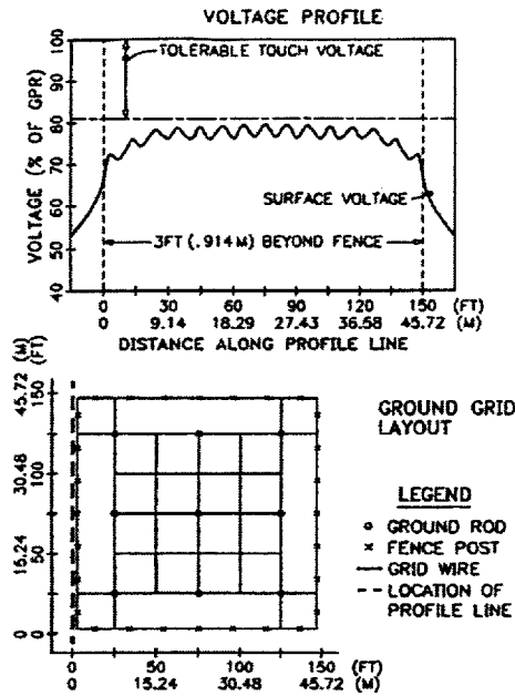
Figure 43—Case 4, plot 1
