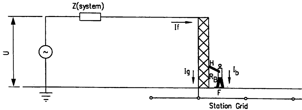
Figure 6—Exposure to touch voltage
