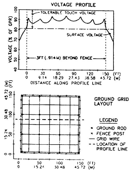
Figure 41—Case 3, plot 1
