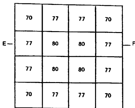
Figure G.4—Measured potential distribution for various ground mats
