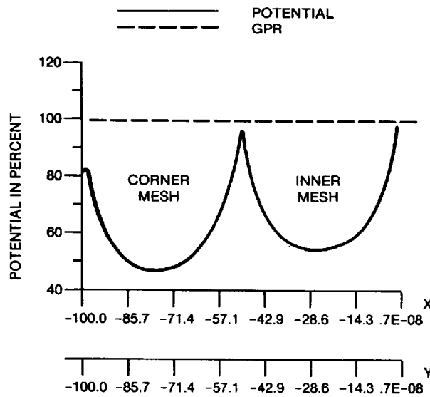
Figure B.6—Diagonal voltage profile for the grid of Figure B.5 in two-layer soil
