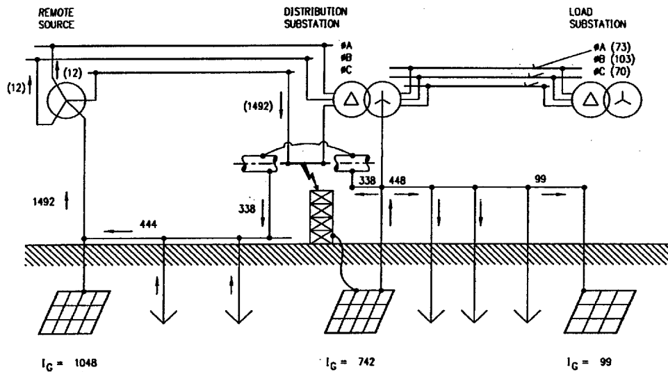
Figure 31—Typical current division for a fault on high side of distribution substation
