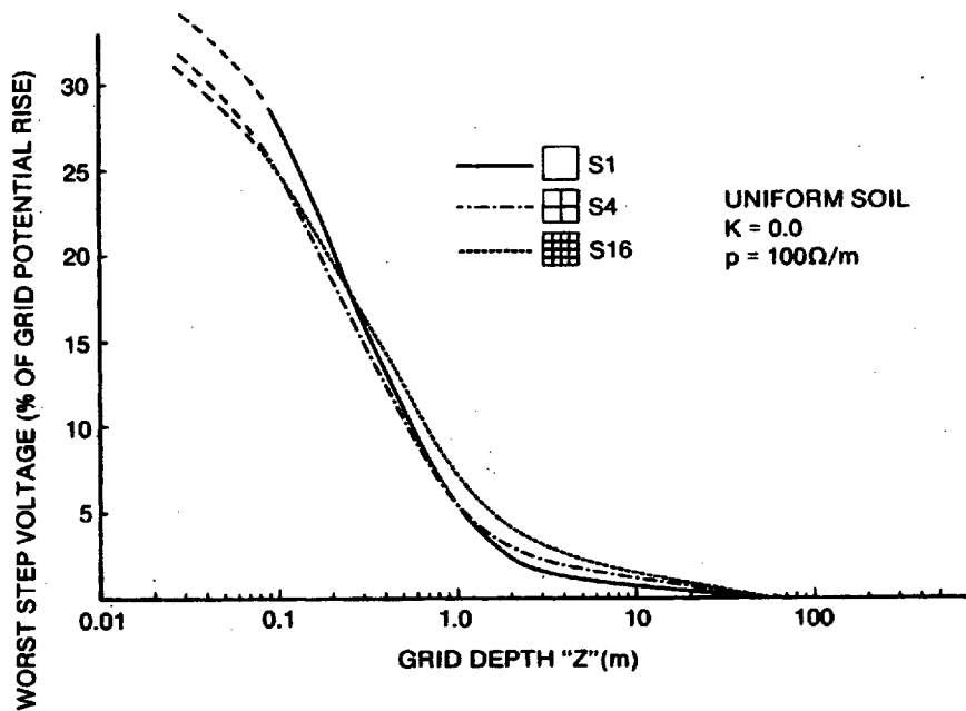
Figure F.11—Step voltage versus grid depth
