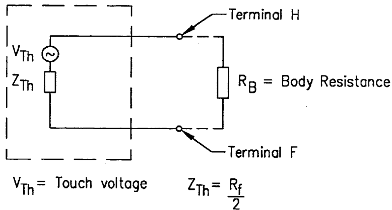
Figure 8—Touch voltage circuit
