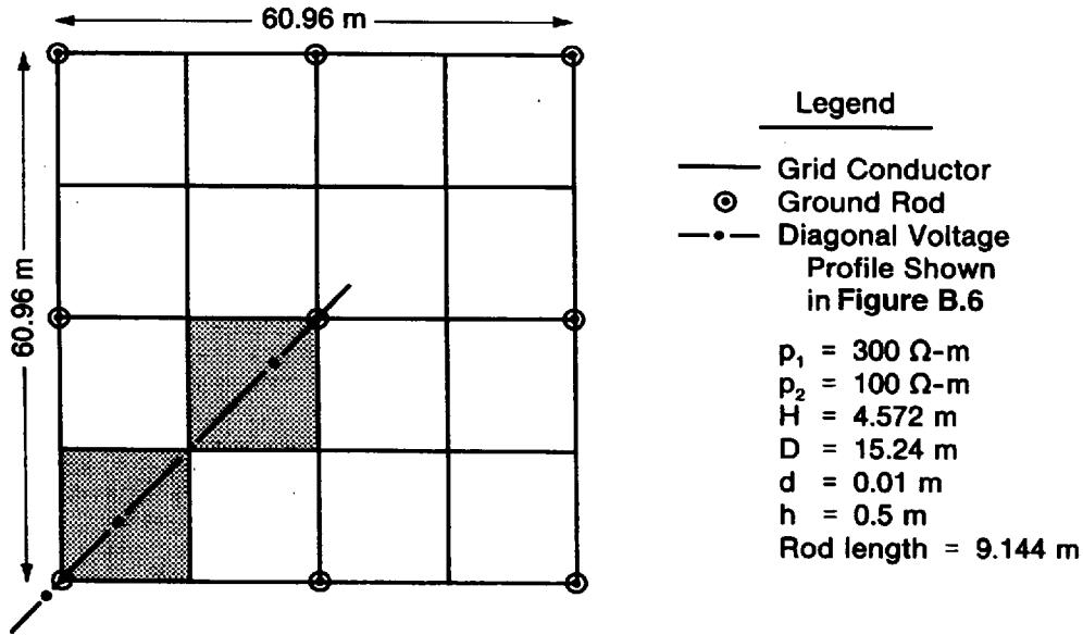
Figure B.5—Equally spaced square grid with nine rods in two-layer soil
