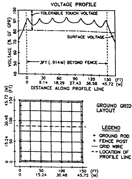
Figure 38—Case 1, plot 2
