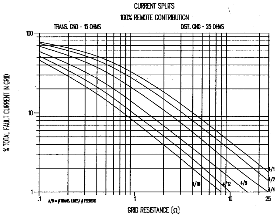
Figure C.5—Curves to approximate split factor S_f
