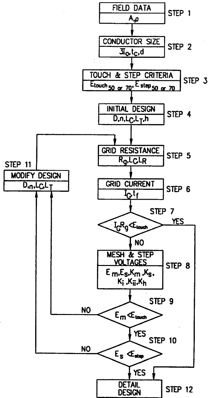
Figure 33—Design procedure block diagram
