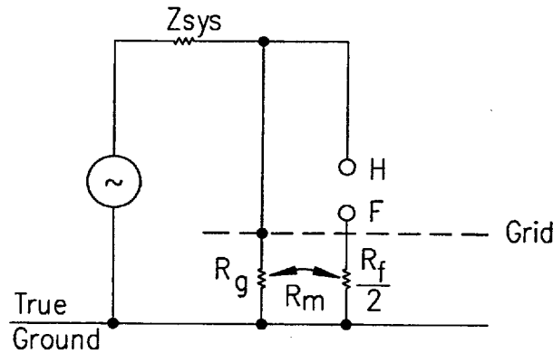
Figure 7—Impedances to touch voltage circuit
